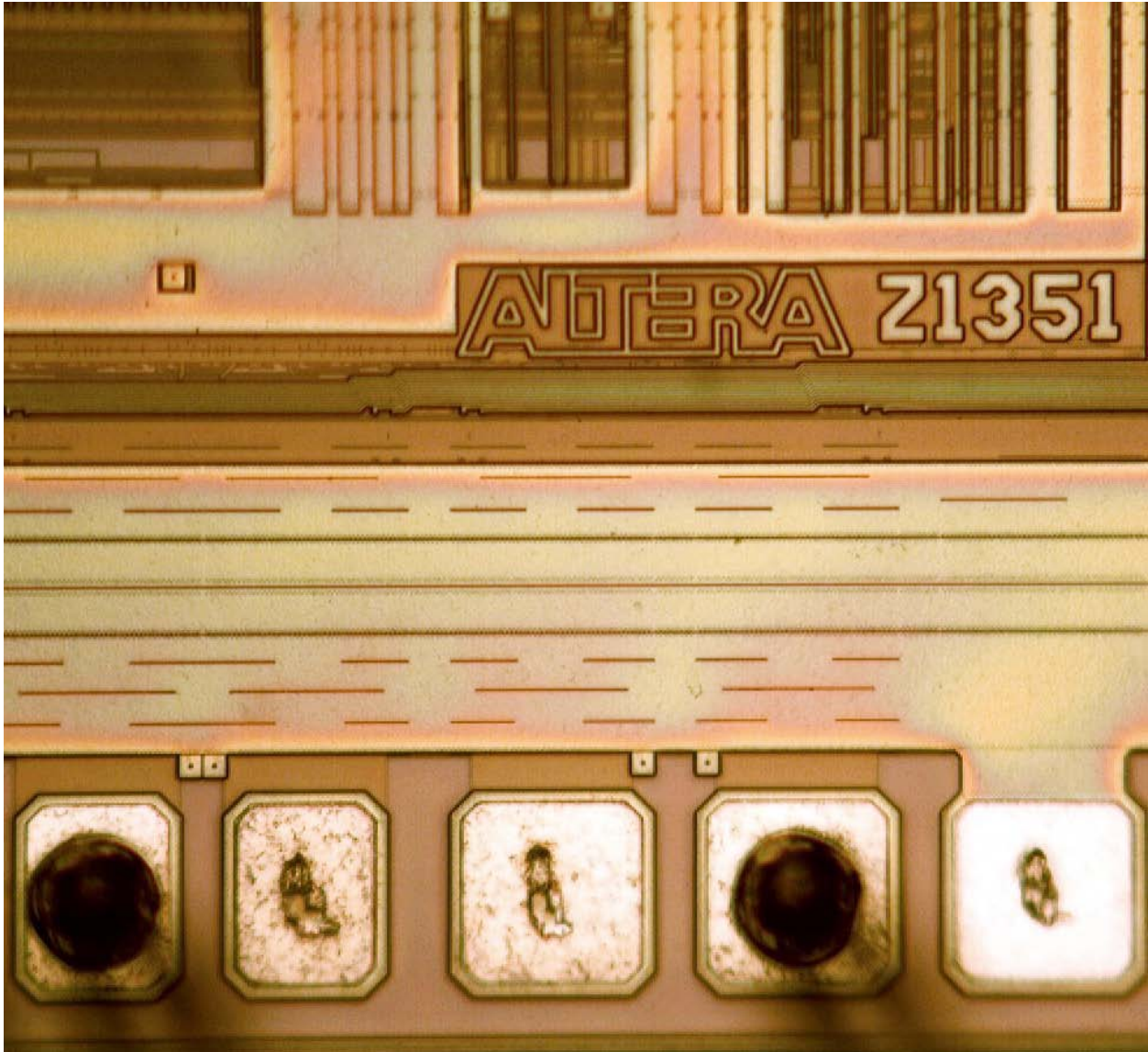
Figure 7 High-Res Metallurgical Image of Die Marking
